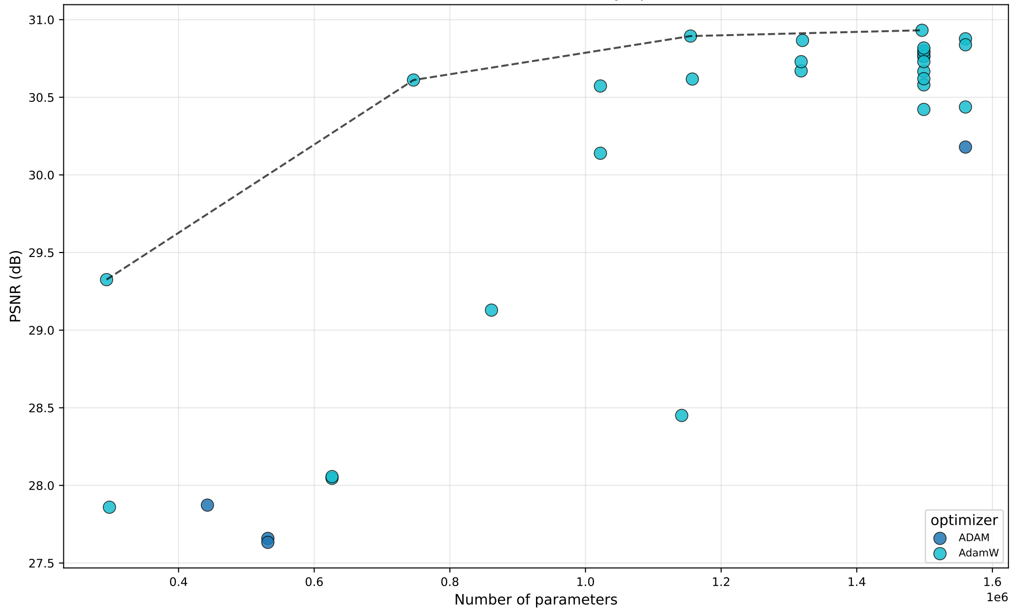
PSNR vs #Params — DAT — by optimizer
